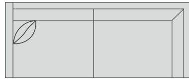
Left Arm Corner Sofa 9DL - 2 W94 D38 H33 Inside Seat W79.5 D22 Standard with 1 P-100 18" Pillow
