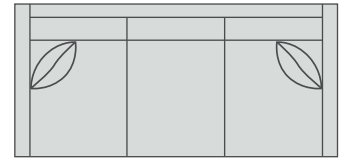
Short Sofa 9B1 - 3 W75.5 D38 H33 Inside Seat W69.5 D22 Standard with 2 P-100 18" Pillows
