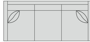
Sofa 9S1 - 3 W85.5 D38 H33 Inside Seat W79.5 D22 Standard with 2 P-100 18" Pillows
