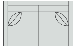
Loveseat 9L1 - 3 W60 D38 H33 Inside Seat W53 D22 Standard with 2 P-100 18" Pillows
