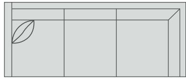
Left Arm Corner Sofa 9DL - 3 W94 D38 H33 Inside Seat W79.5 D22 Standard with 1 P-100 18" Pillow
