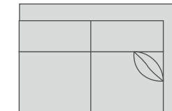
4901-LR Amy Right Arm Loveseat W56.5 D39 H37 Inside Seat W52 D22
